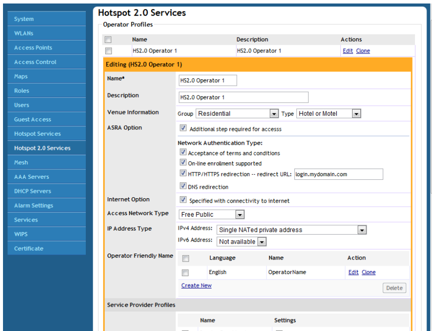
Figure 127. Creating a Hotspot 2.0 Operator Profile
