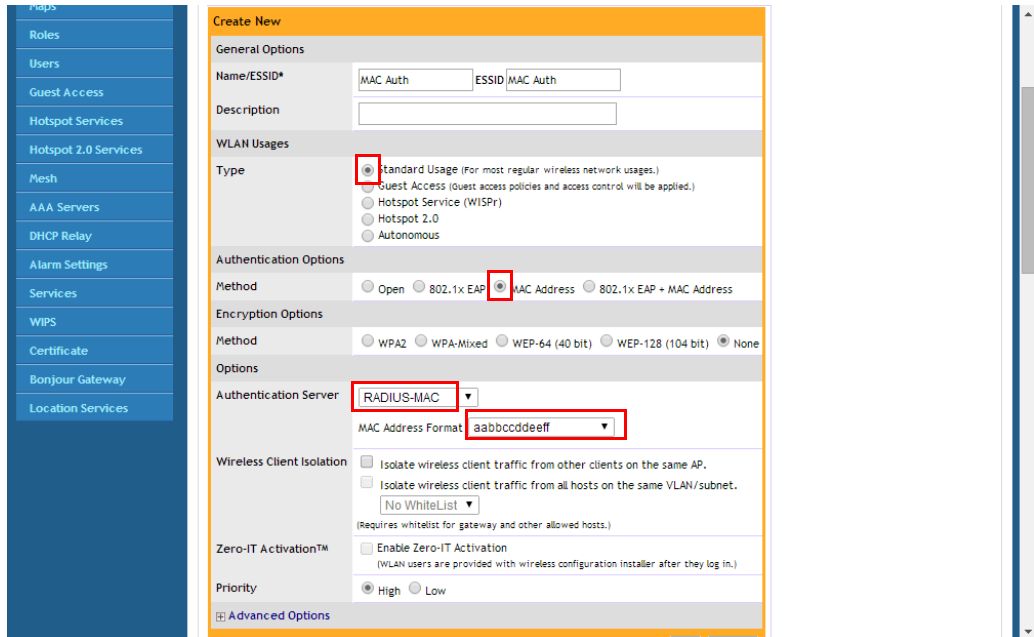
Figure 101. RADIUS authentication using MAC address
