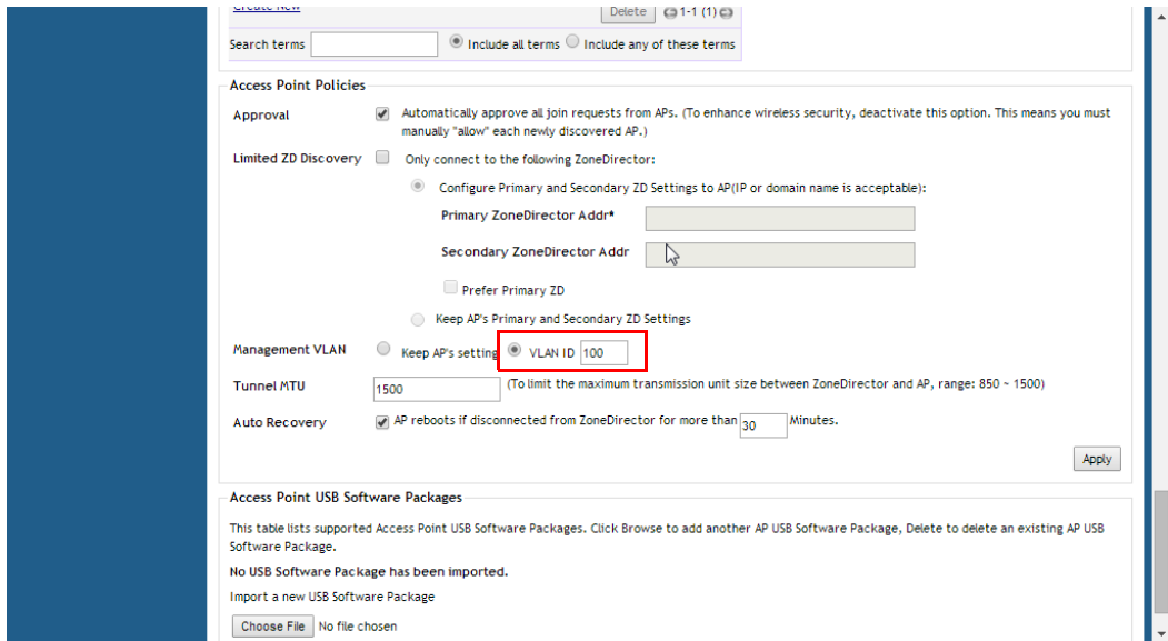
Figure 119. Configuring management VLAN for APs
