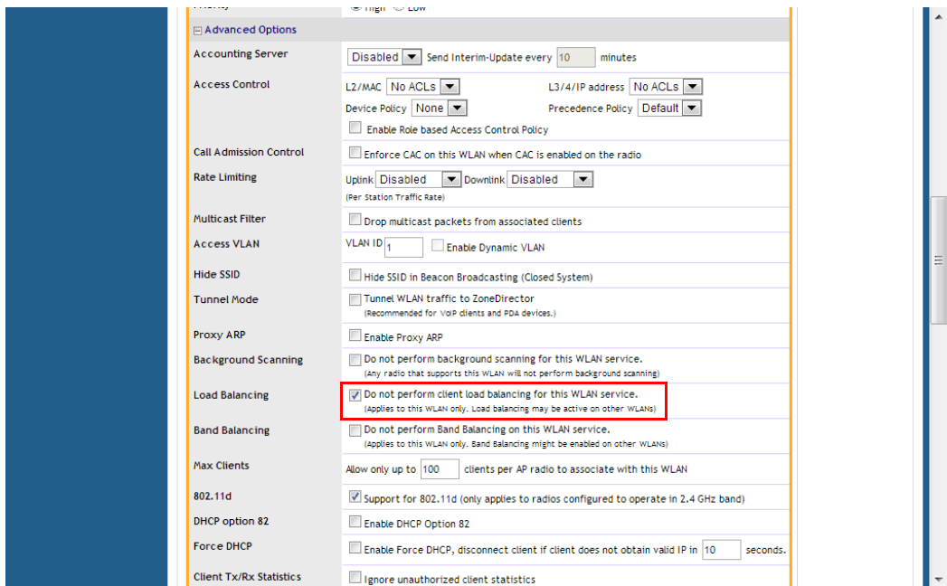
Figure 67. Disable load balancing on a specific WLAN
