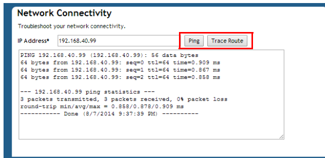
Figure 247. Network Connectivity dialog
