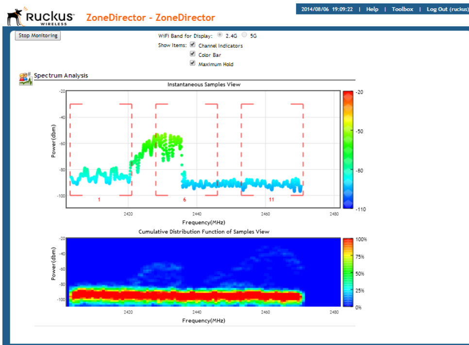
Figure 169. The Spectrum Analysis page
