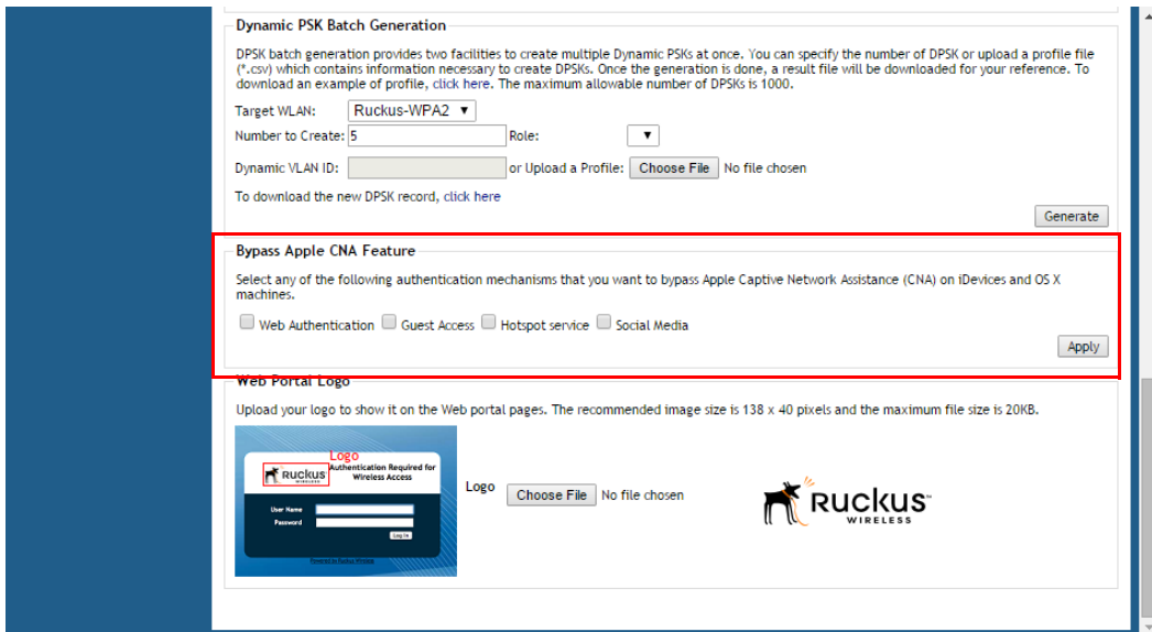
Figure 134. Enabling the Bypass Apple CNA Feature
