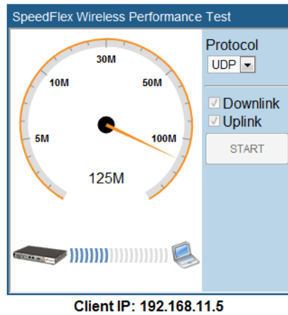
Figure 241. A progress bar appears as SpeedFlex measures the wireless throughput
