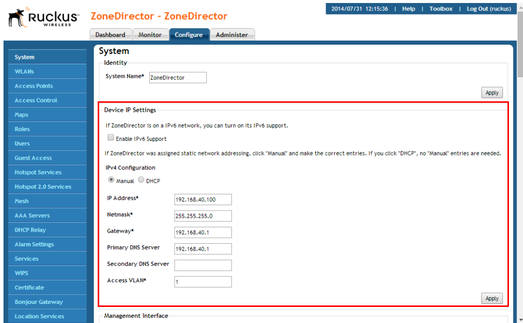
Figure 23. The Device IP options
