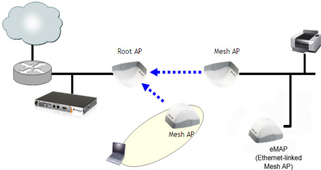
Figure 221. eMAP - Hybrid Mesh topology
