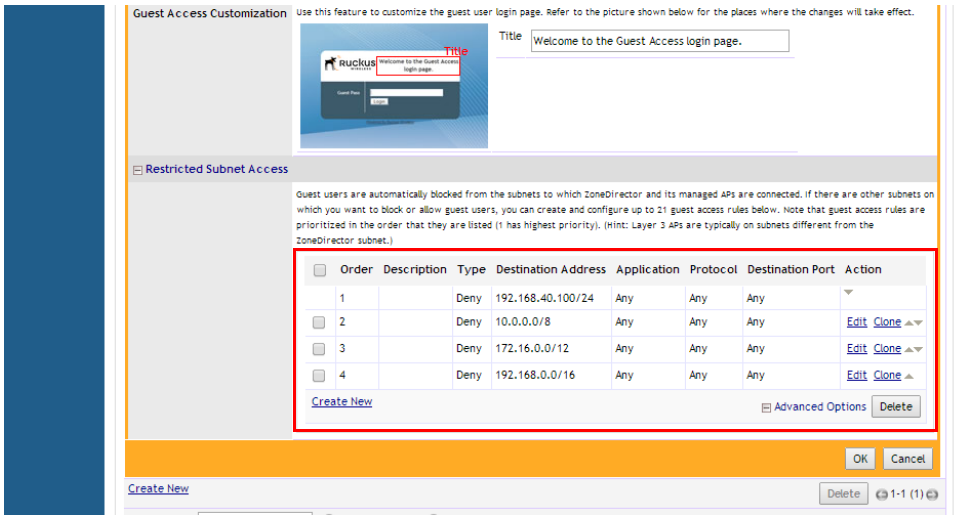
Figure 203. The Restricted Subnet Access options
