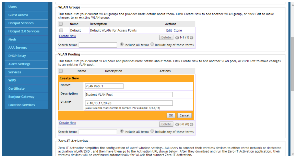
Figure 121. Creating a VLAN pool
