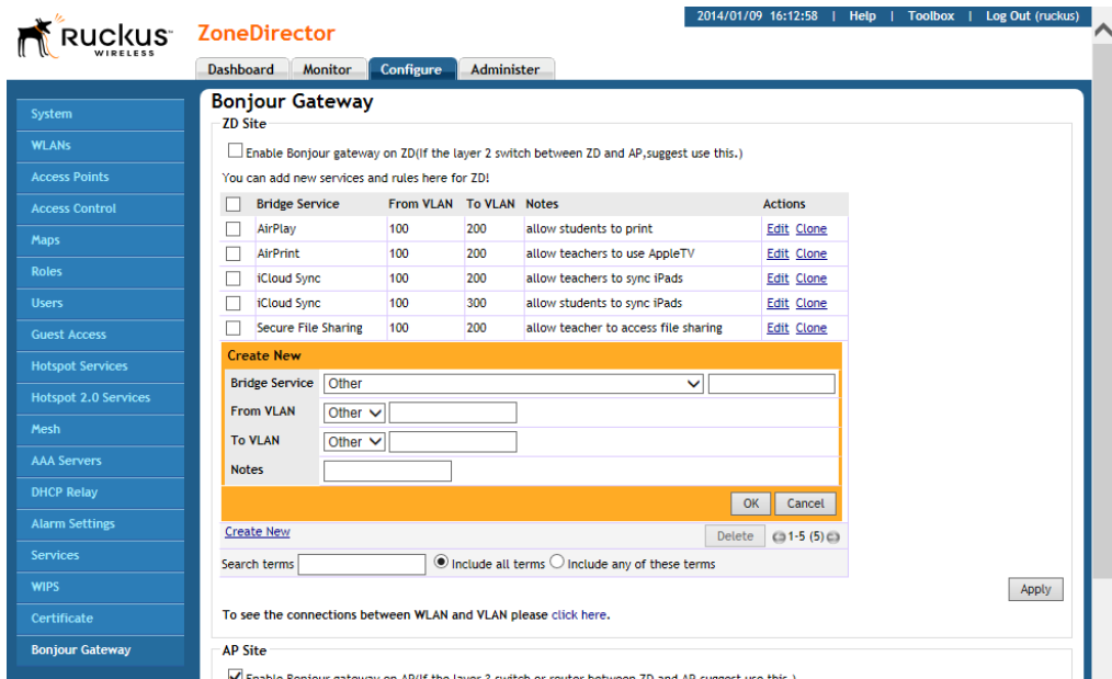
Figure 56. Creating a ZD Site Bonjour Gateway rule
