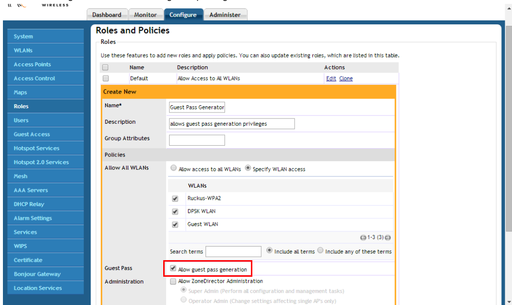
Figure 210. Create a guest pass generator Role
