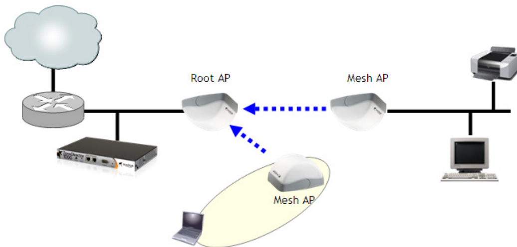
Figure 220. Mesh - wireless bridge topology
