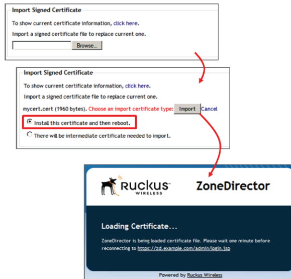
Figure 233. Importing a signed SSL Certificate
