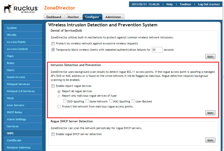
Figure 77. Intrusion Prevention options
