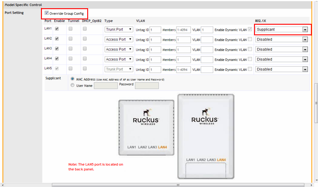
Figure 144. Configuring an AP Ethernet port as an 802.1X Supplicant
