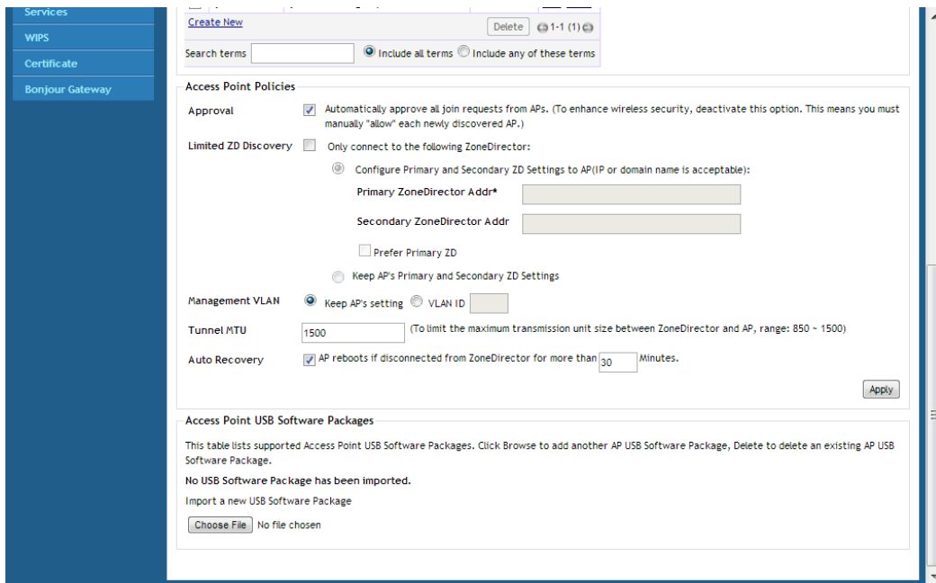
Figure 146. Setting global AP policies on the Configure > Access Points page
