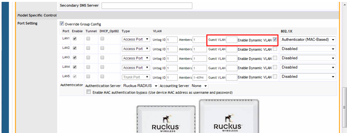
Figure 143. Enabling Guest VLAN and Dynamic VLAN on a MAC-based 802.1X Authenticator port
