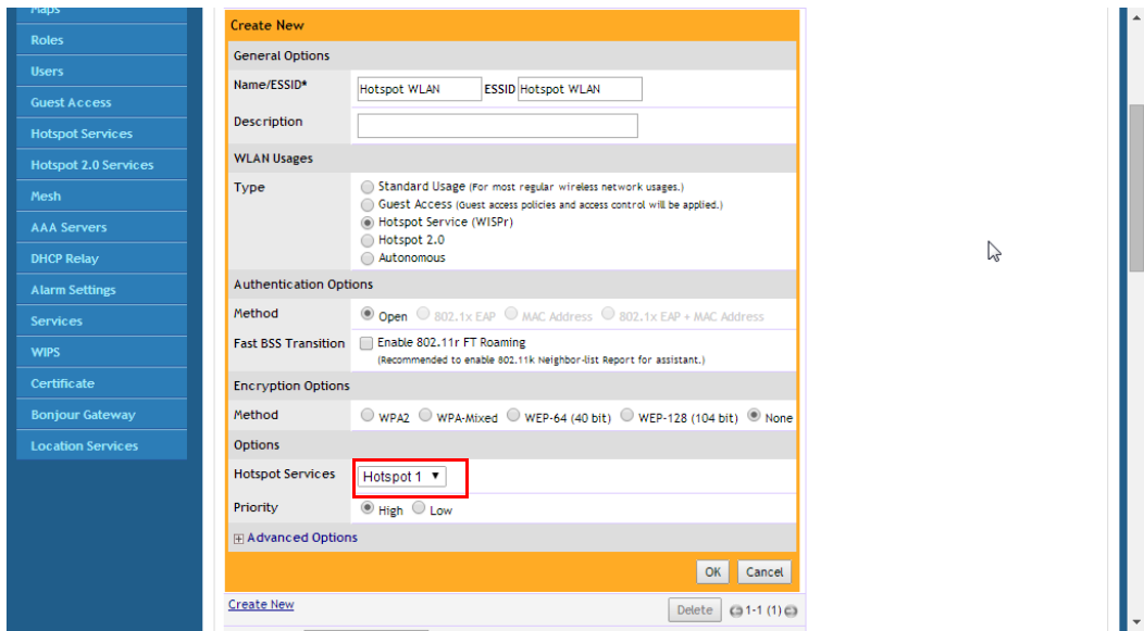
Figure 124. Assigning a Hotspot service to a Hotspot WLAN
