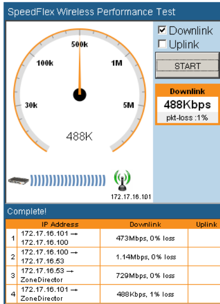
Figure 244. Multi-Hop SpeedFlex test results
