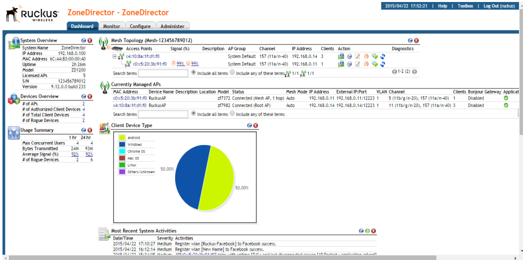
Figure 12. The Dashboard
