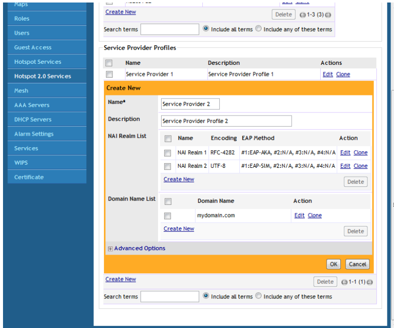
Figure 125. Creating a Service Provider Profile
