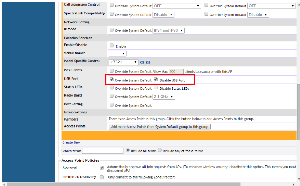
Figure 139. Disabling AP USB ports
