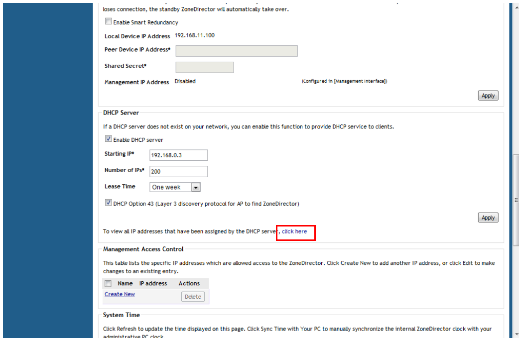
Figure 35. To view current DHCP clients, click the “click here” link
