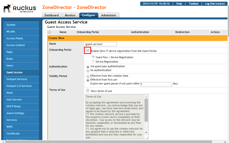
Figure 205. Enable Onboarding Portal
