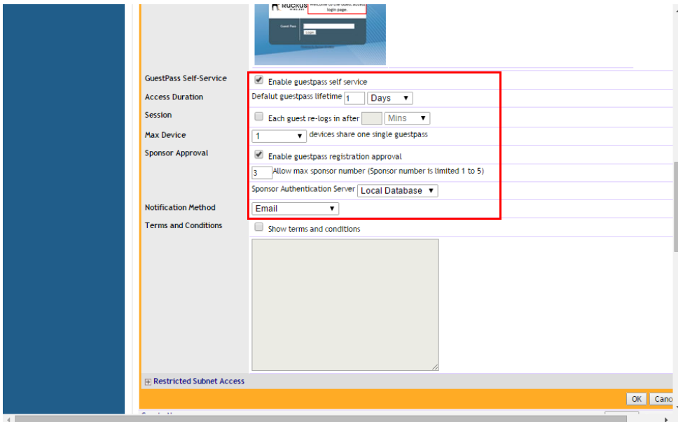
Figure 189. Creating a Self-Service Guest Access service
