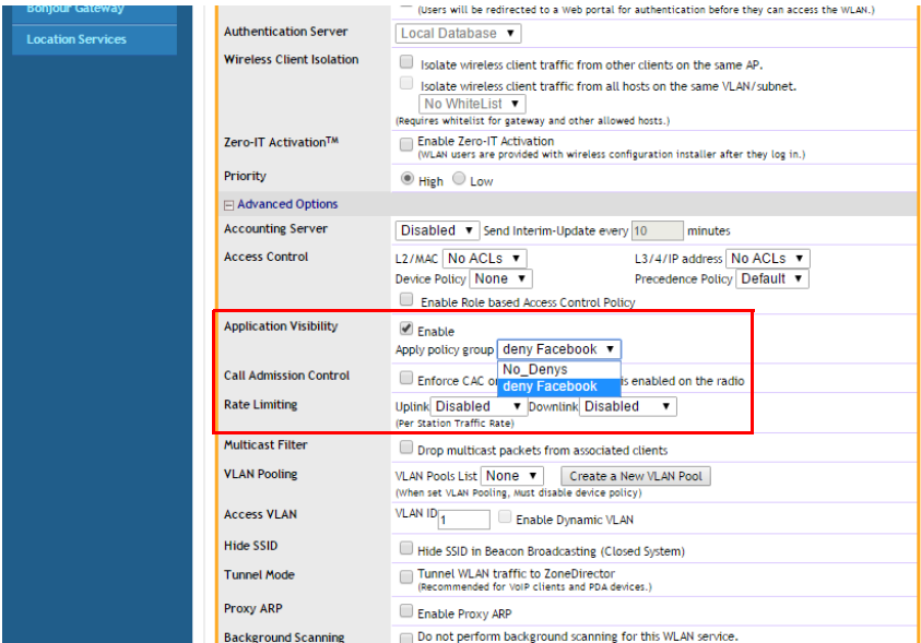
Figure 93. Apply an Application Denial Policy to a WLAN
