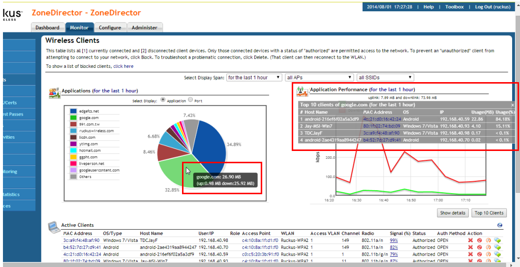
Figure 158. Viewing the top 10 clients of an application
